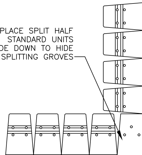
ODD COURSES
