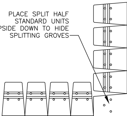
EVEN COURSES
