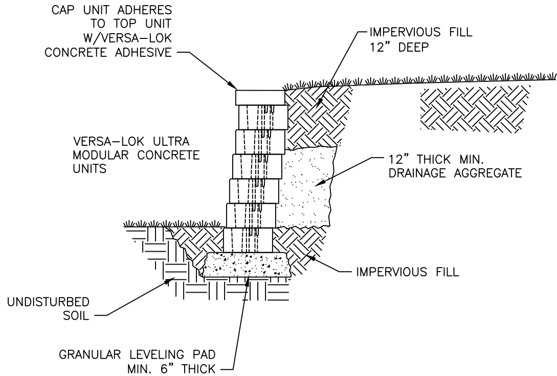
TYPICAL SECTION – UNREINFORCED RETAINING WALL SCALE: 1/2"=1'
